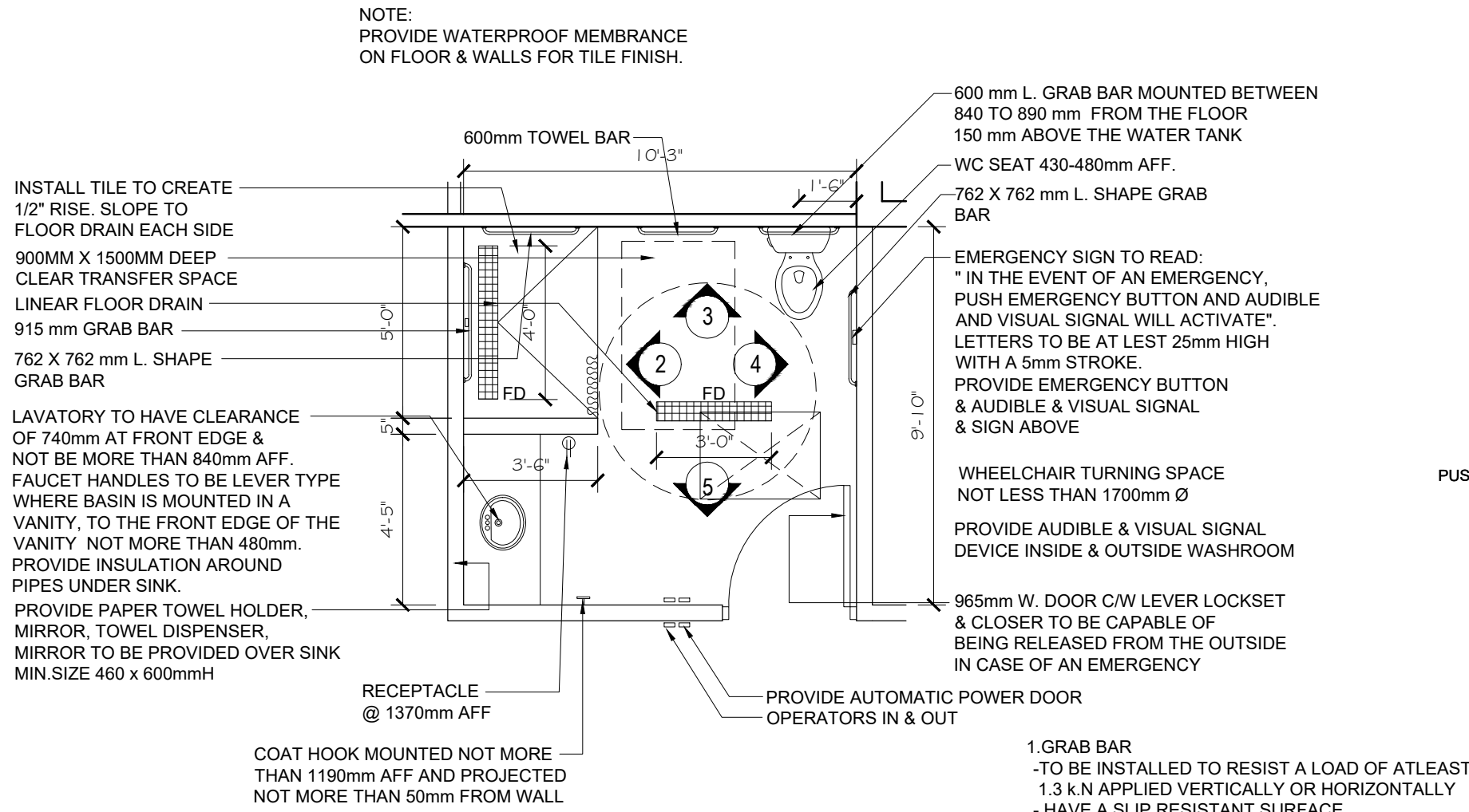
1 HC WASHROOM PLAN-RM17 SCALE 1/4" = 1' - 0"
